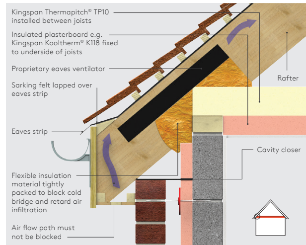
Figure 9a - Ventilated loft floor detail at eaves
