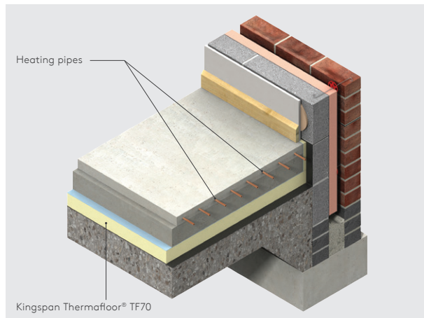
Figure 6 - 24 Hour heating applications - below the floor slab
